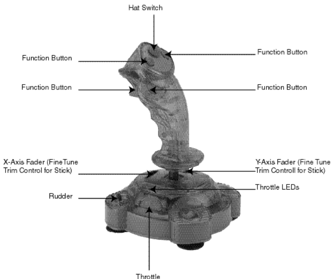
Figure 1 - Button/Switch Operation
